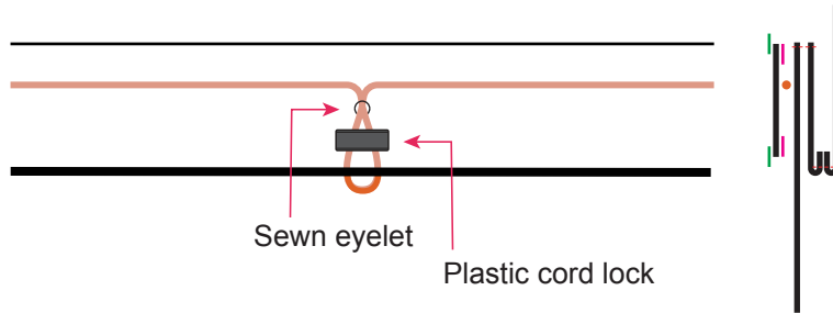
CB HOOD - EXTERIOR X-RAY BACK OF HOOD SHOCK CORD- CORD LOCK
